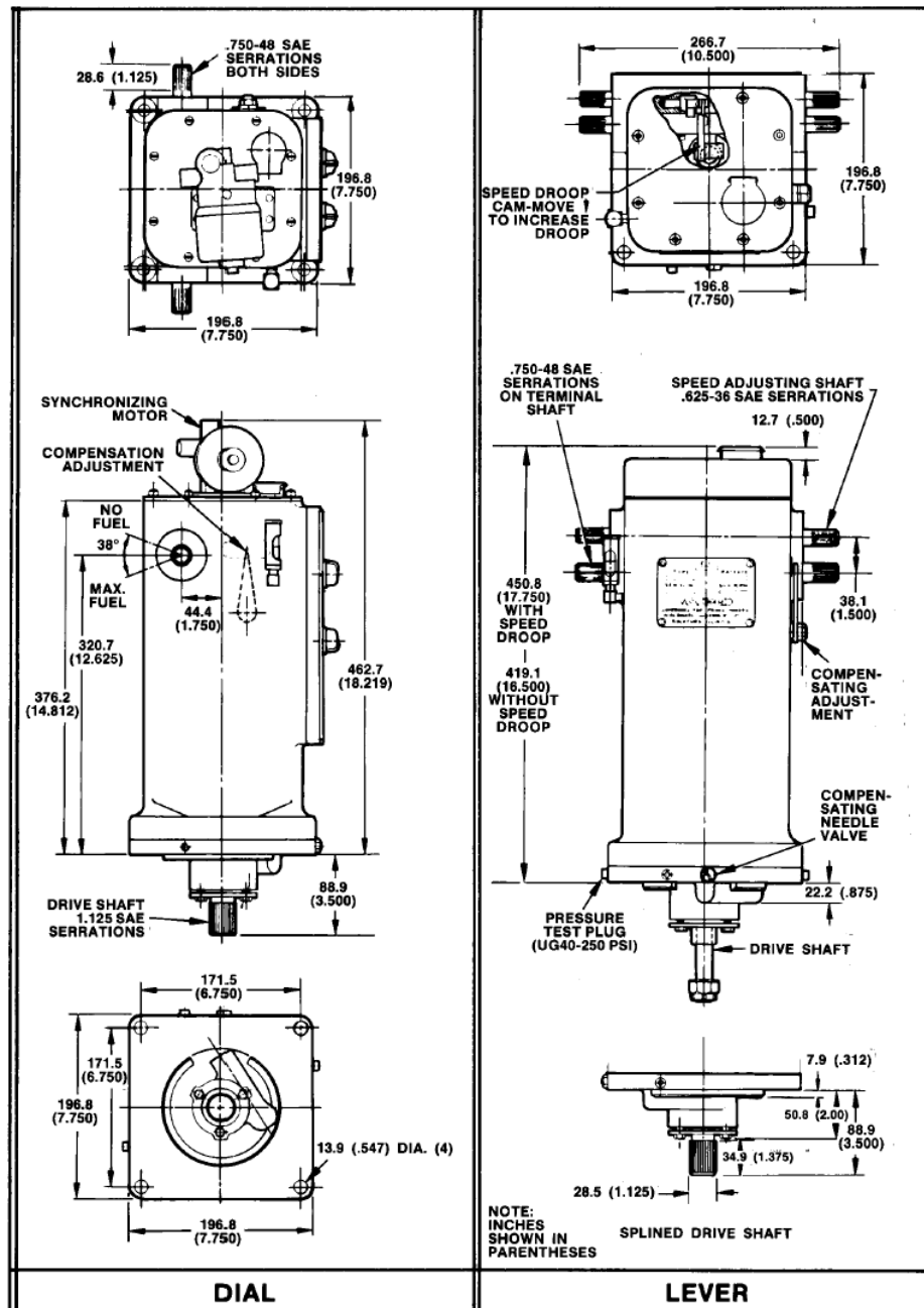
UG-40 Governors (Do not use for construction)
